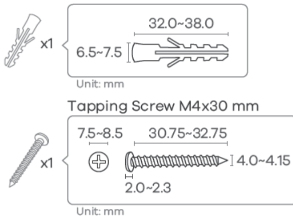
Figure 19 WX5600-T0 / WX3100 Screw Specifications
