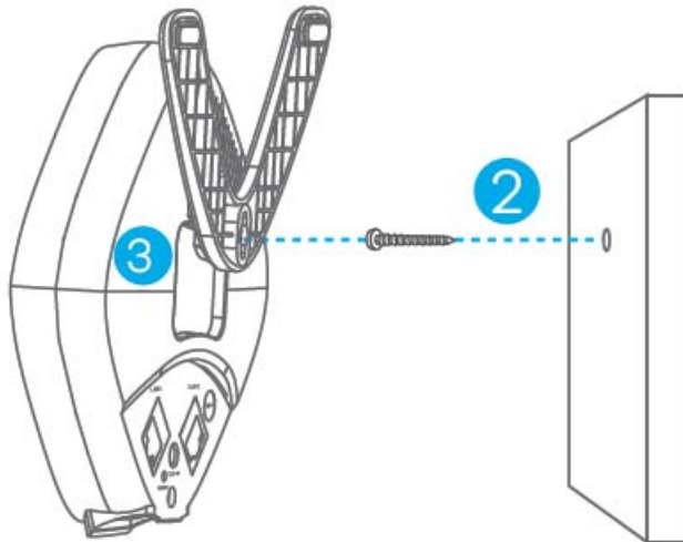
Figure 21 Wall Mounting
