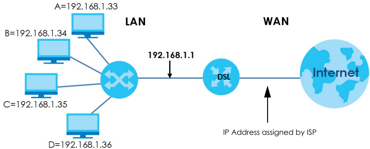
Figure 145 Multiple Servers Behind NAT Example
