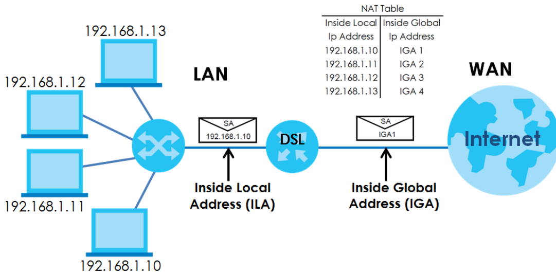
Figure 143 How NAT Works
