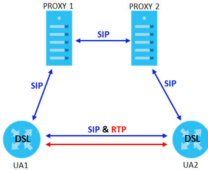
Figure 200 SIP Call Through Proxy Servers
