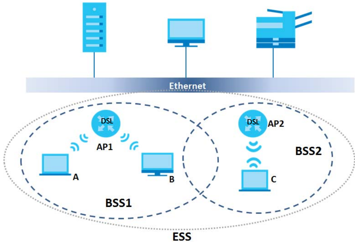
Figure 244 Infrastructure WLAN
