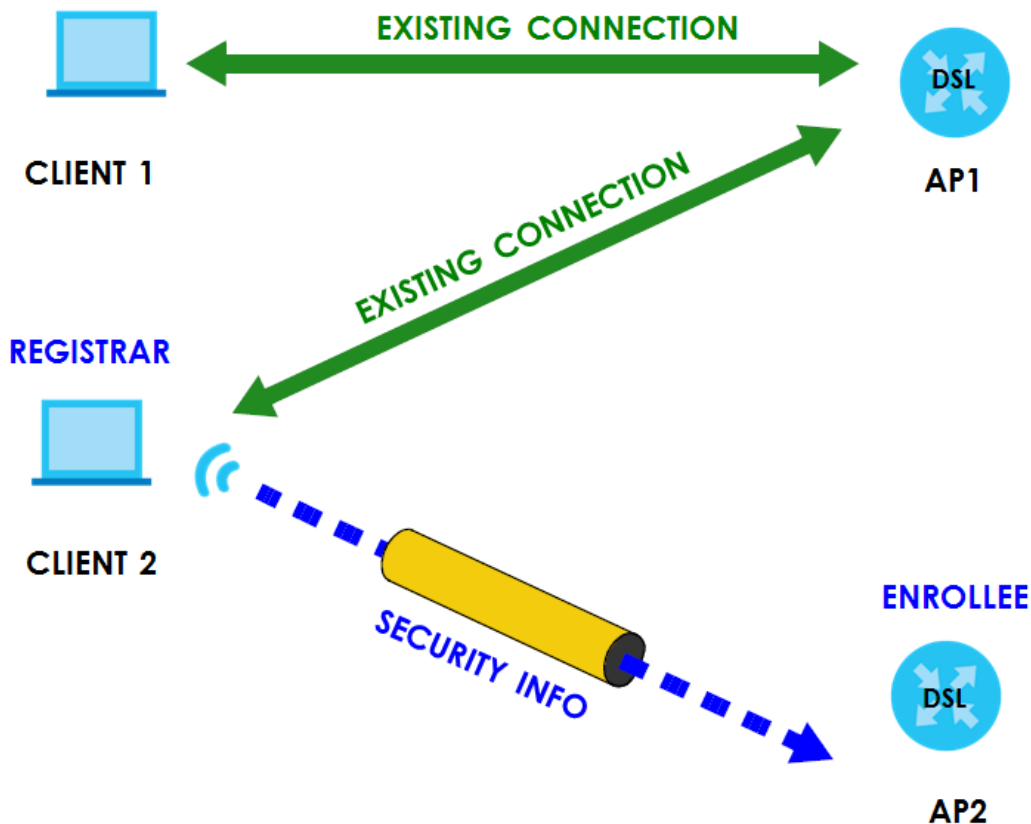
Figure 105 WPS: Example Network Step 3
