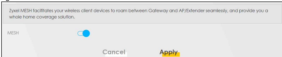
Figure 96 Network &gt; Wireless &gt; MESH
