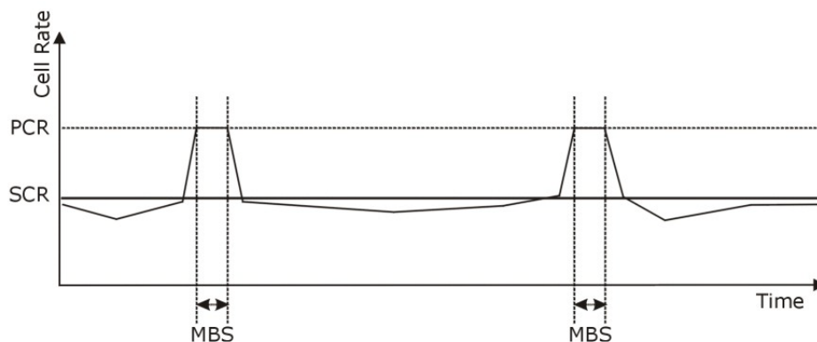
Figure 83 Example of Traffic Shaping
