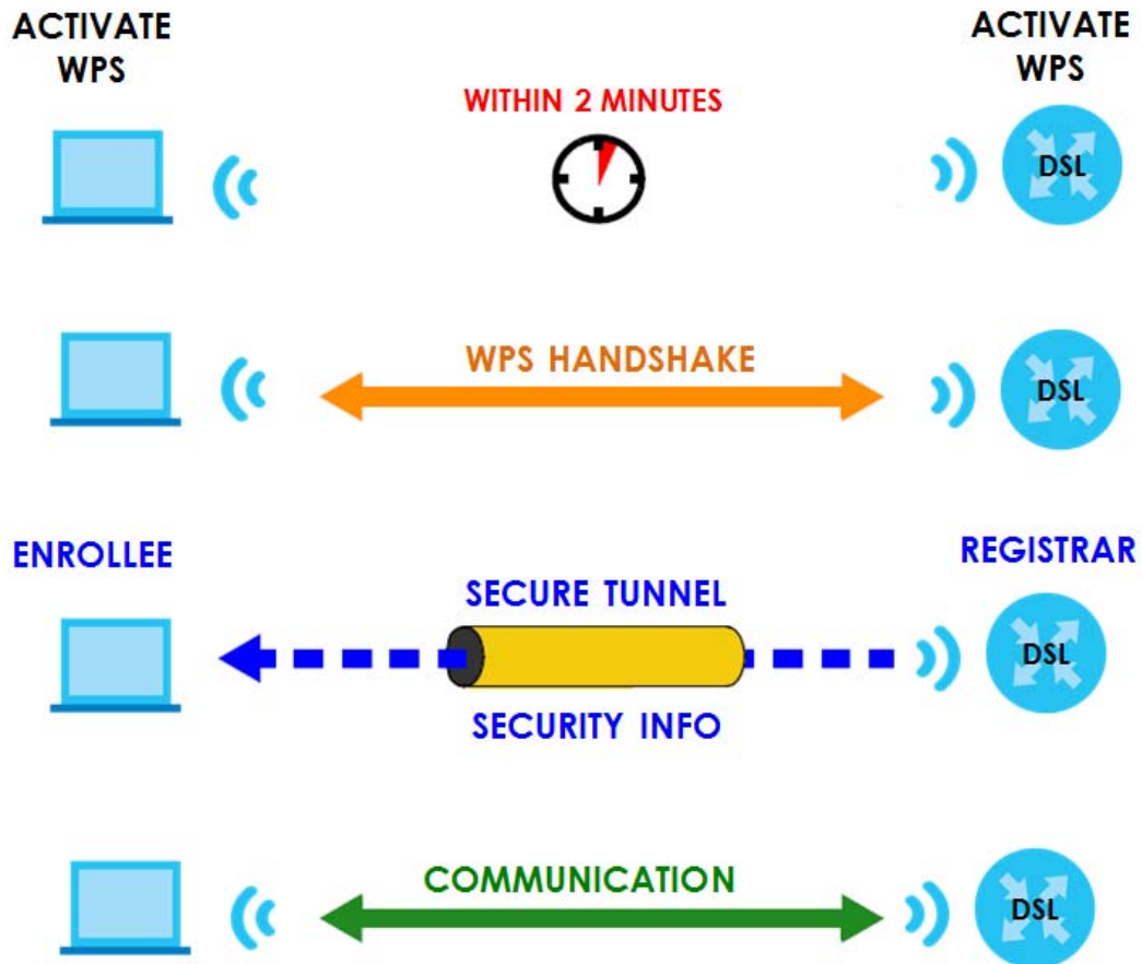
Figure 102 How WPS works
