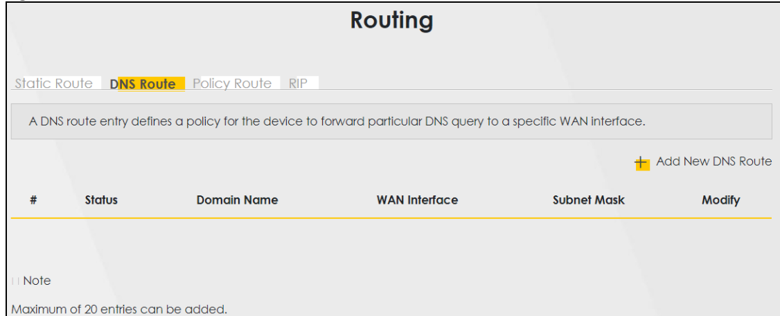
Figure 118 Network Setting > Routing > DNS Route
