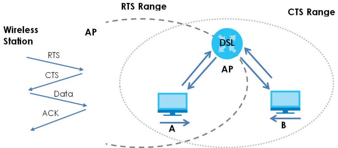
Figure 245 RTS/CTS
