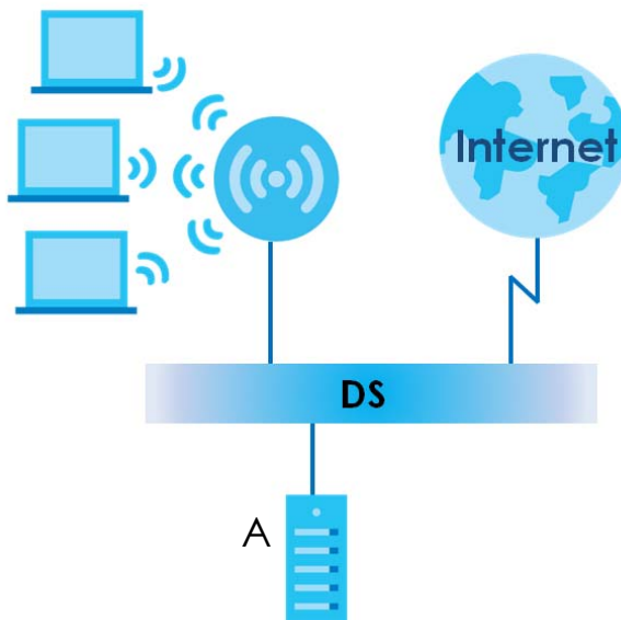
Figure 246 WPA(2) with RADIUS Application Example
