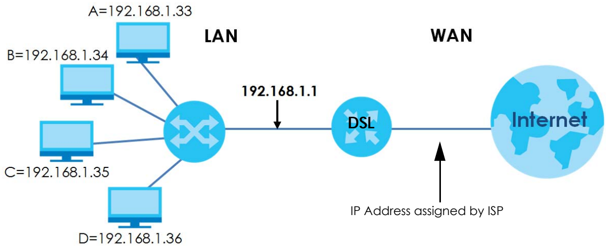
Figure 132 Multiple Servers Behind NAT Example
