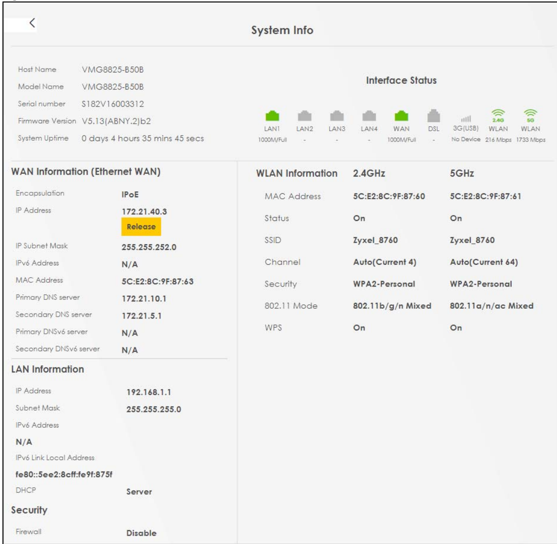
Figure 58 System Info: Detailed Information
