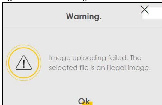
Figure 230 Error Message
