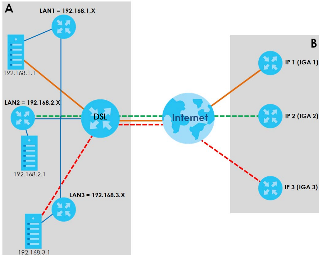
Figure 144 NAT Application With IP Alias
