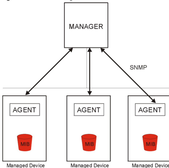
Figure 221 SNMP Management Model
