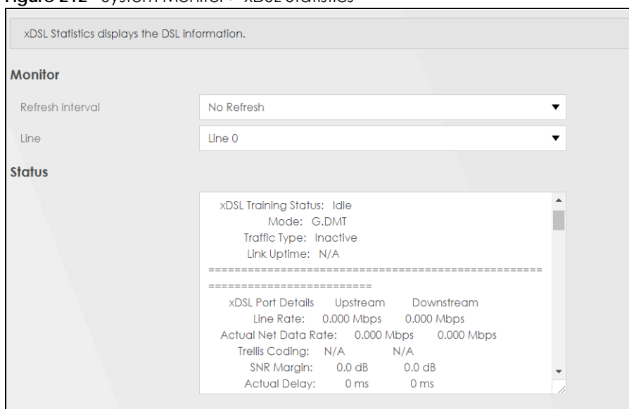
Figure 212 System Monitor > xDSL Statistics
